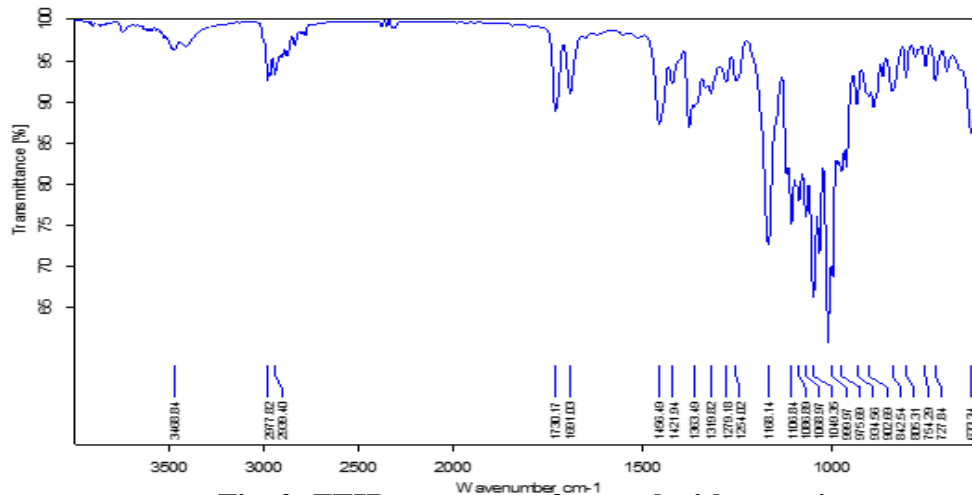
Fig. 2: FTIR spectrum of pure clarithromycin
