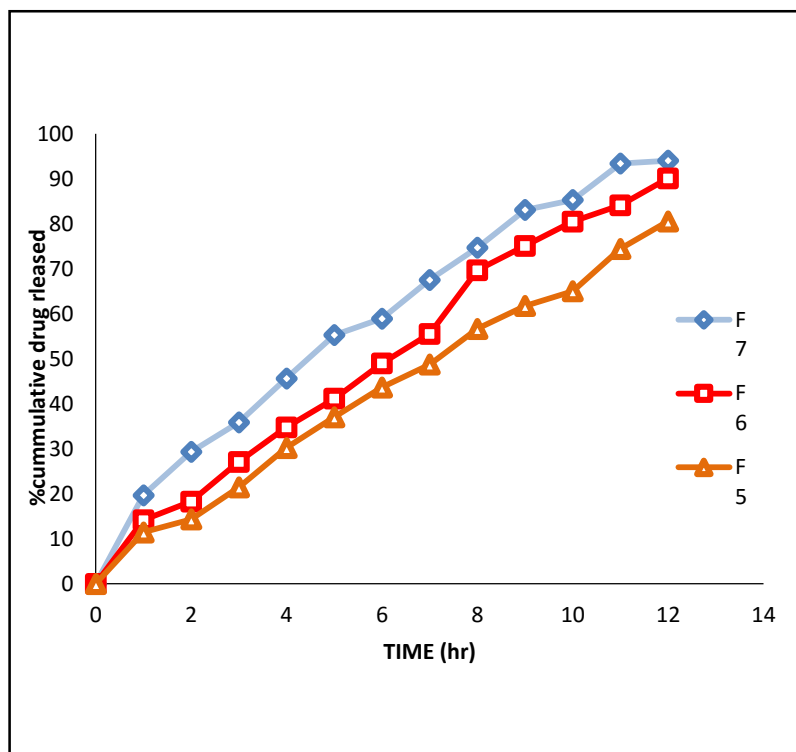
Fig. 4: In vitro drug release of (F5-F7)
