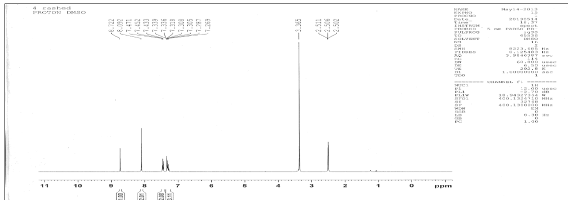
Fig.(4):H-NMR spectrum of compound(3).
