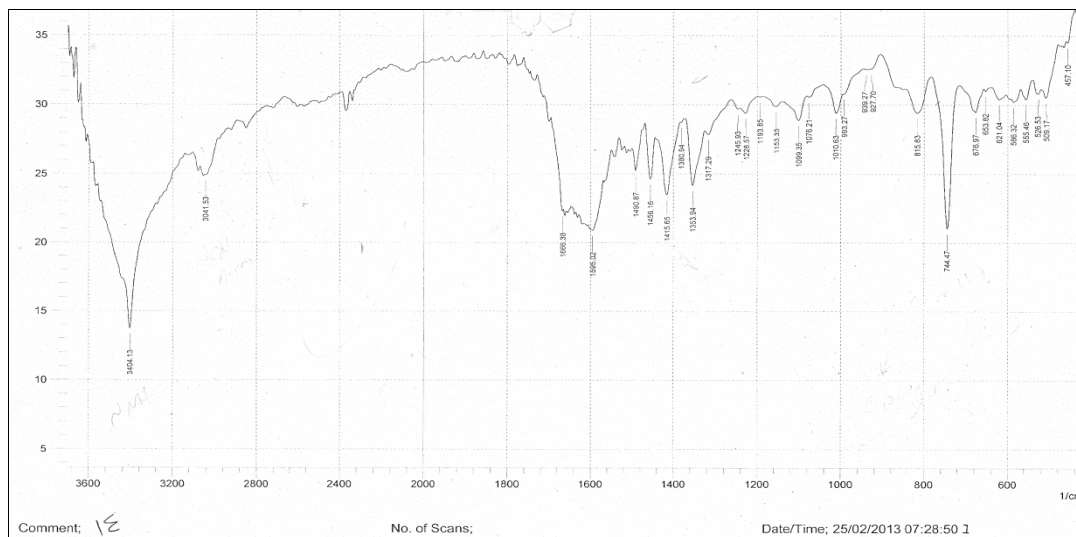
Fig.(10): 1 H-NMR spectrum of compound(9).
