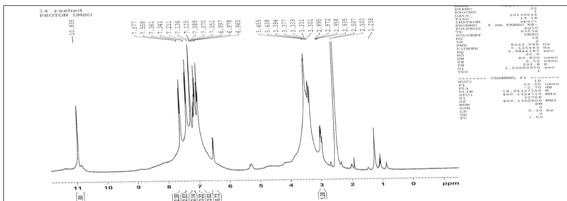
Fig.(13):H-NMR spectrum of compound(11).
