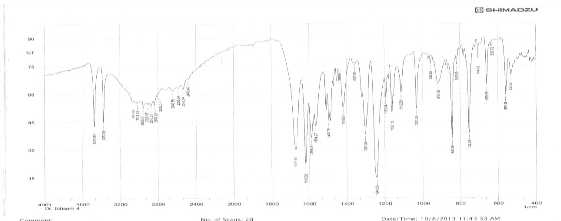
Fig.(12):FT-IR spectrum of compound(15).
