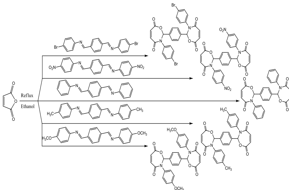
Scheme 2: represents oxazepines compounds(6-10).
