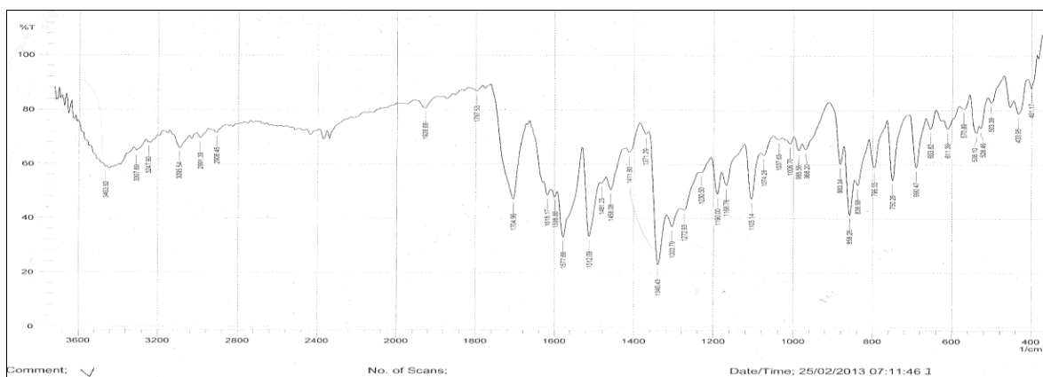
Fig.(7):FT-IR spectrum of compound(7).
