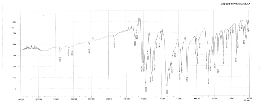
Fig.(1):FT-IR spectrum of compound(1).
