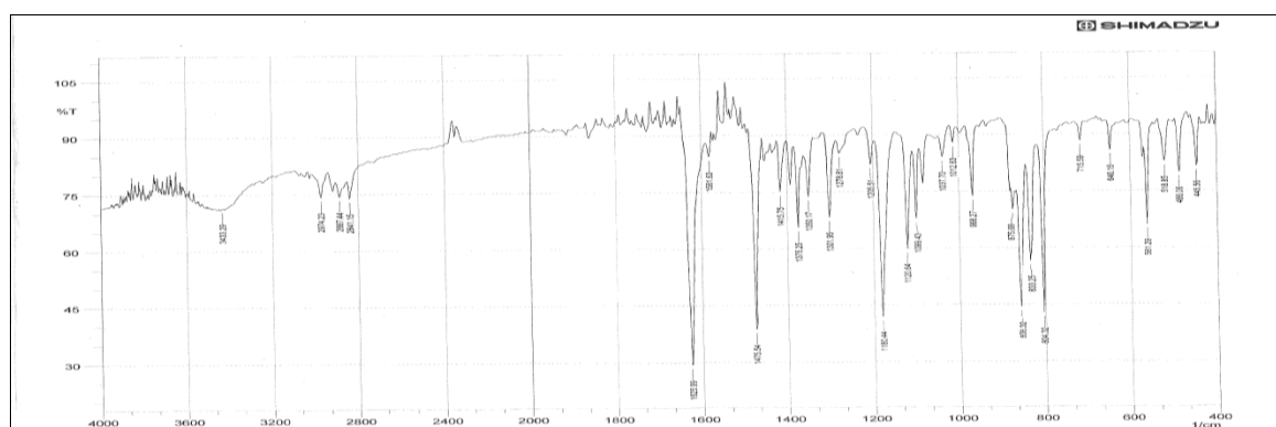
Fig.(1):FT-IR spectrum of compound(1).
