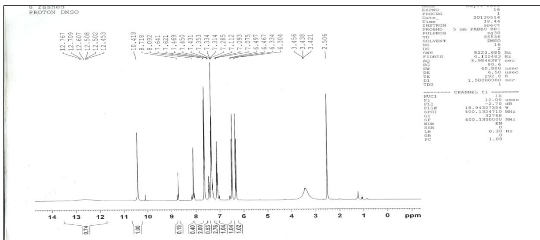
Fig.(10): 1 H-NMR spectrum of compound(9).
