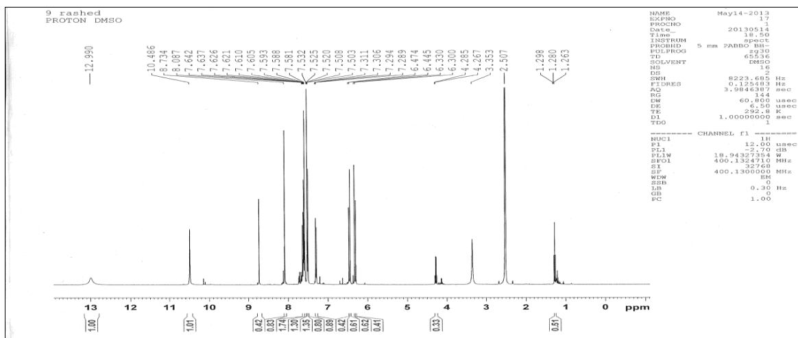
Fig.(8):H-NMR spectrum of compound(6).
