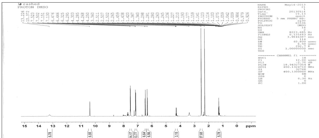
Fig.(9): 1 H-NMR spectrum of compound(8).
