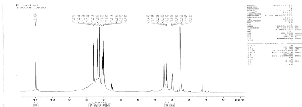
Fig.(14):H-NMR spectrum of compound(13).
