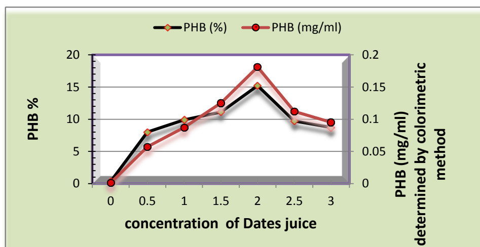
Fig.5: Effect of Carbon Sources (Dates juice) concentration in bacteria growth and PHB accumulation by Bacillus spp. in production medium and condition according of find in (2.5.4).
