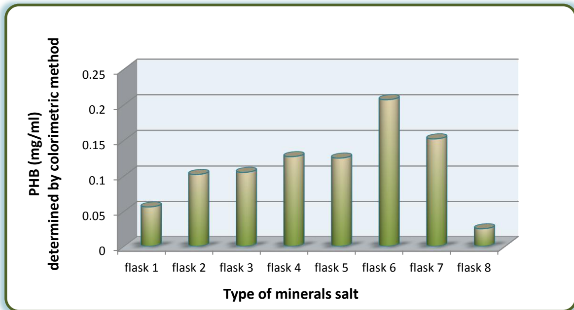
Fig.8: Effect of of different multivalent minerals in bacteria growth and PHB accumulation by Bacillus spp. in production medium and condition according of find in (2.5.6).
