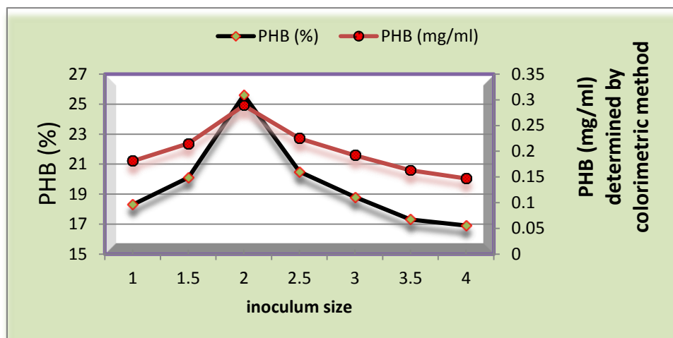
Fig.11: Effect of inoculum size in bacteria growth and PHB accumulation by Bacillus spp. in production medium and condition according of find in (2.5.8).
