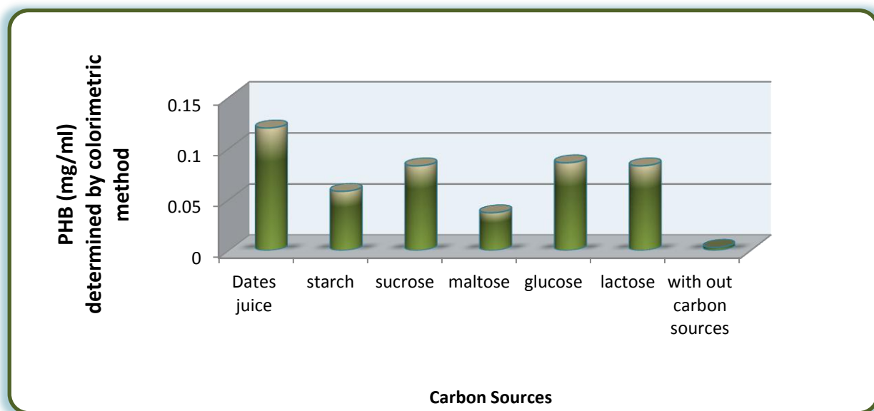
Fig.4: Effect of Carbon Sources in bacteria growth and PHB accumulation by Bacillus spp. in production medium and condition according of find in (2.5.4).
