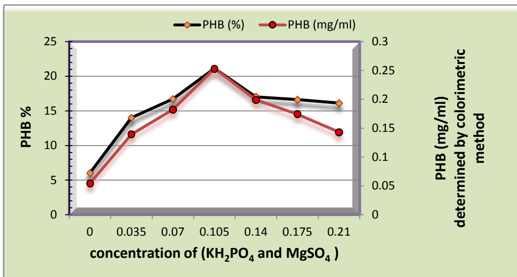
Fig.9: Effect of different ( \text{KH}_2\text{PO}_4 and \text{MgSO}_4 ) concentration in bacteria growth and PHB accumulation by Bacillus spp. in production medium and condition according of find in (2.5.6).
