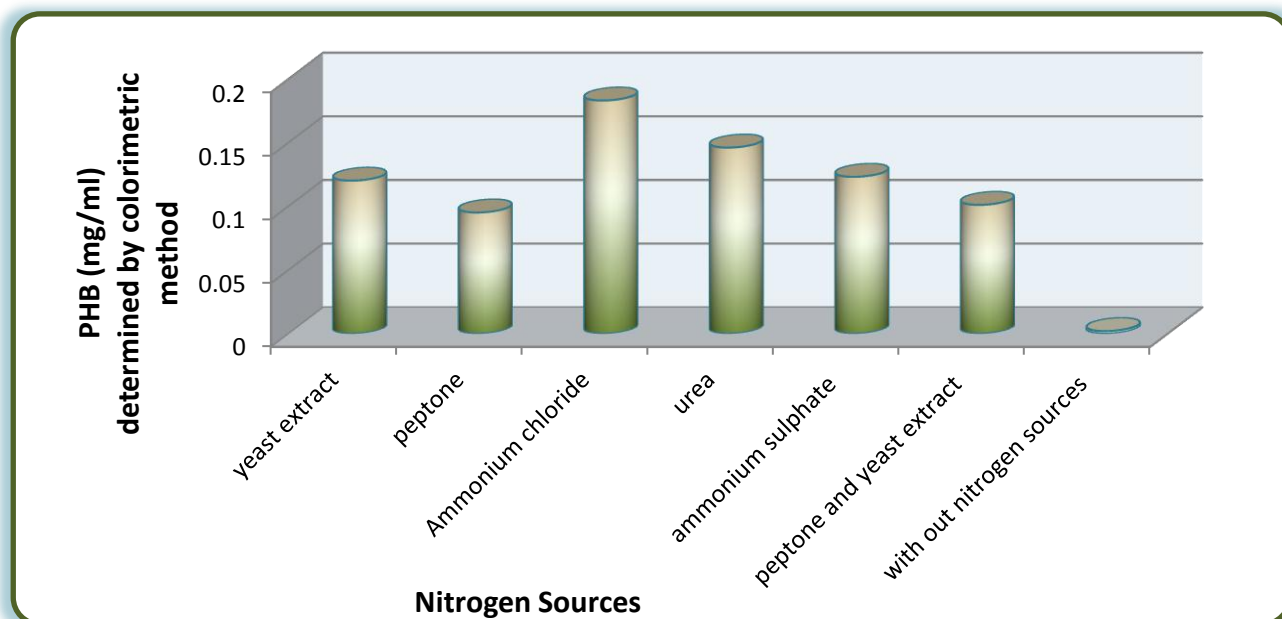
Fig.6: Effect of Nitrogen Sources in bacteria growth and PHB accumulation by Bacillus spp. in production medium and condition according of find in (2.5.5).
