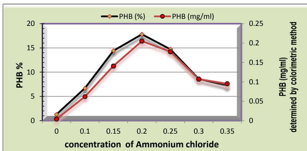
Fig.6: Effect of Nitrogen Sources in bacteria growth and PHB accumulation by Bacillus spp. in production medium and condition according of find in (2.5.5).
