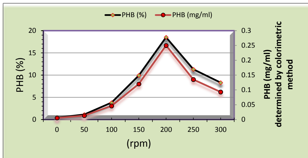
Fig.3: Effect of rotational speed in bacteria growth and PHB accumulation by Bacillus spp. in production medium and condition according of find in (2.5.3).
