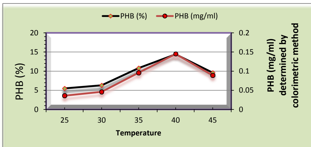
Fig.2: Effect of Incubation Temperature in bacteria growth and PHB accumulation by Bacillus spp. in production medium and condition according of find in (2.5.2).
