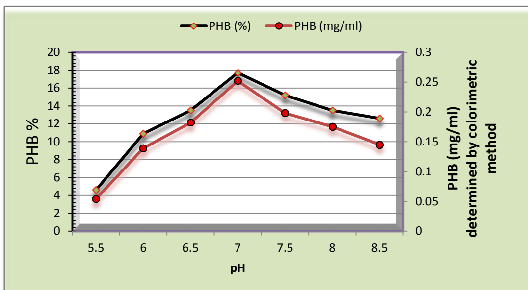
Fig.10: Effect of pH in bacteria growth and PHB accumulation by Bacillus spp. in production medium and condition according of find in (2.5.7).
