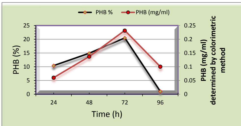
Fig. 1: Effect of Incubation time in bacteria growth and PHB accumulation by Bacillus spp. in production medium and condition according of find in (2.5.1).
