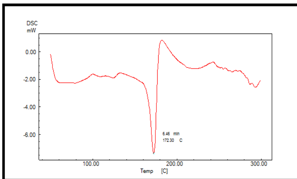
Figure 4. DSC thermogram of pure candesartan cilexetil
