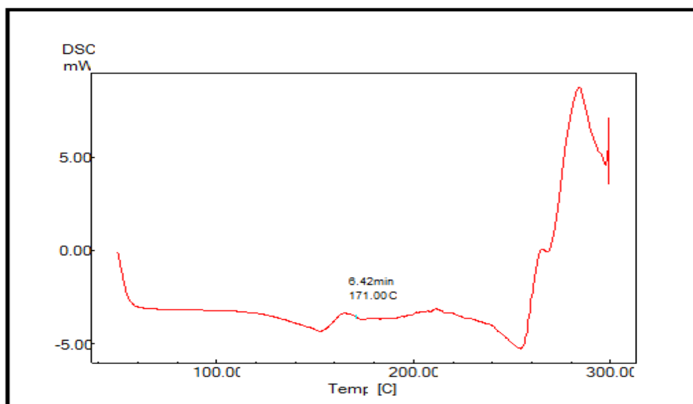
Figure 6. DSC thermogram of F2 (poloxamer) nanoparticles
