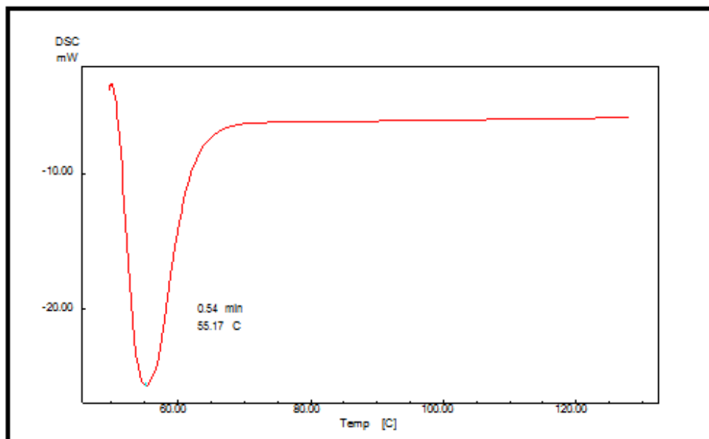
Figure 5. DSC thermogram of pure Poloxamer
