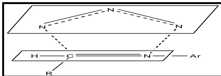
Scheme: Approximate transition state geometry for azide addition.
