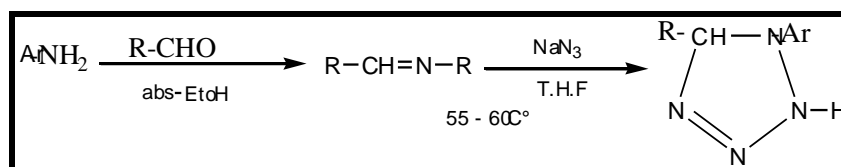
Scheme : Regents and conditions of the preparation of tetrazole.[4]
