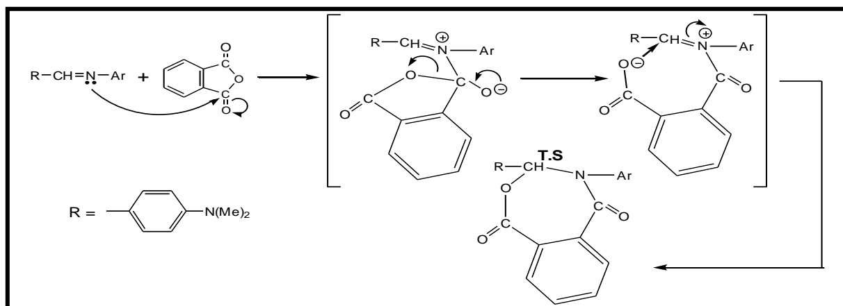
Scheme , Mechanism steps for the prepared compounds [6,7].
