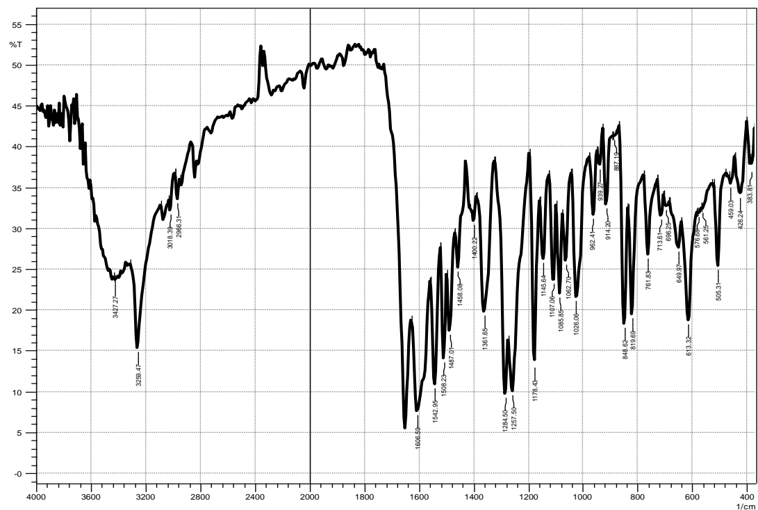
Figure.(2) IR spectral for compound (IV 7 )
