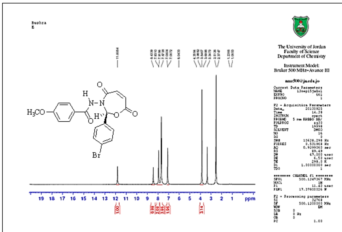
Figure.(7) 1 H NMR for compound(IV 10 )
