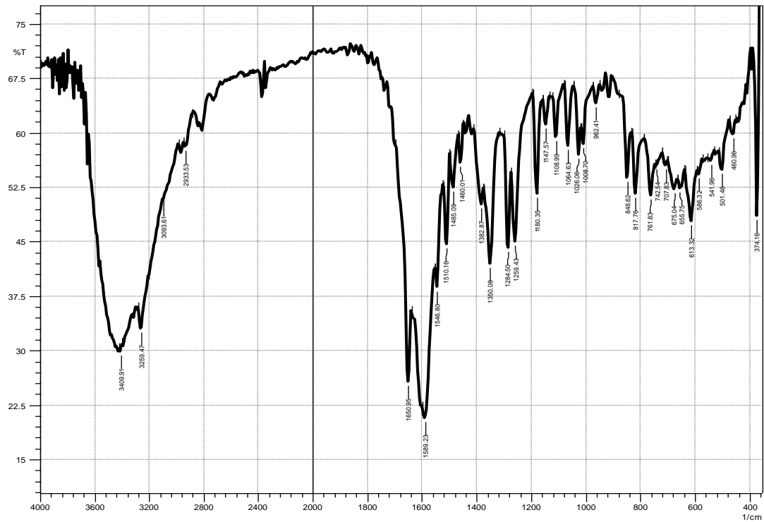
Figure.(3) IR spectral for compound (IV 10 )
