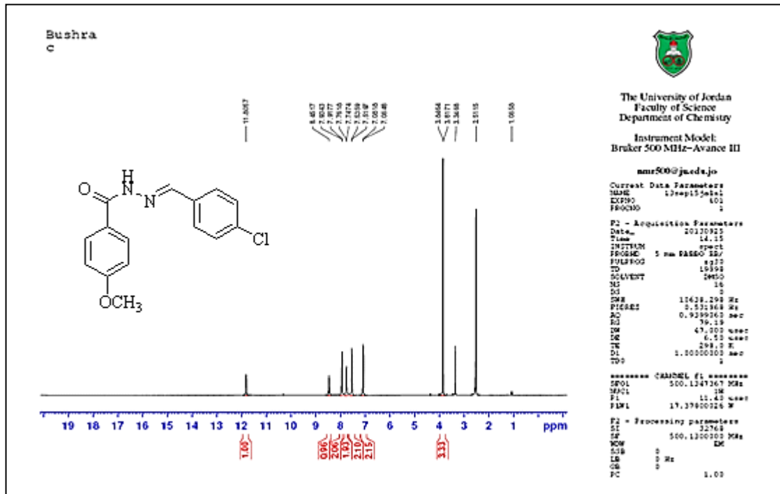
Figure.(5) 1 HNMR for compound(III 3 )
