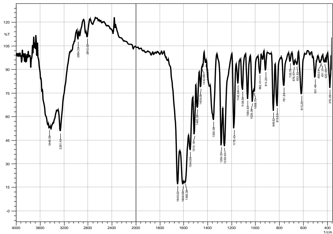
Figure.(1) IR spectral for compound(III 5 )
