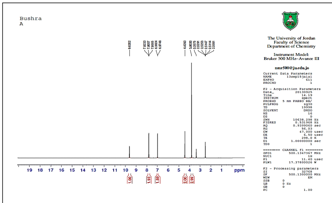
Figure.(4) 1 H NMR for compound(II 2 )
