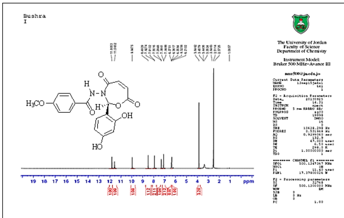
Figure.(6) 1 HNMR for compound(IV 9 )
